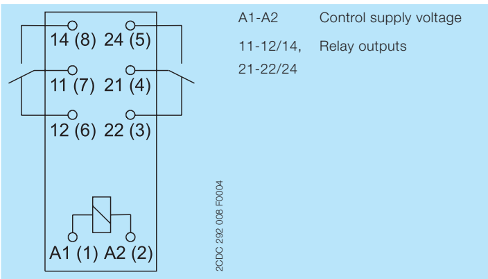
Connection diagram
