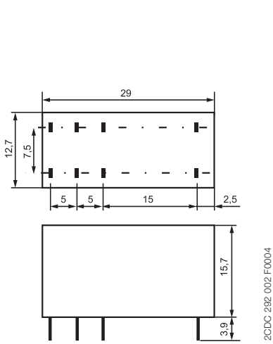
CR-P relays
