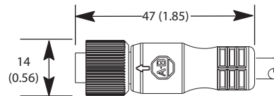
Straight Female M12 Quick Disconnect
