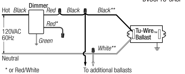
Wiring Diagram 10 Single-Pole Wiring
