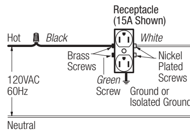
Wiring Diagram 7 Receptacle Wiring
