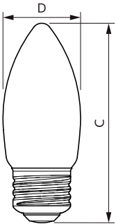
Candle B11 120V 4.5?-40W 300lm 2700-2200
