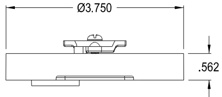
ASSEMBLY OF FSC405R W/ 5/8" WINGS
