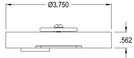
ASSEMBLY OF FSC405R W/ 1/2" WINGS
