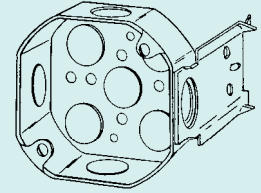
40JB-1/2 1-1/2" Deep JB bracket set flush, gauging notches 3/8" & 1/2"
