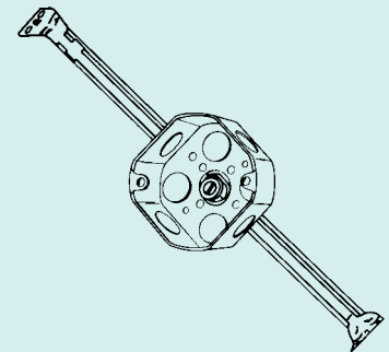
SX115-40-1/2 1-1/2" Deep 40-1/2 box on SX115 stud bar hanger adjusts from 11-1/2" to 18-1/2"
