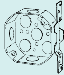
40VB-1/2 1-1/2" Deep Vertical bracket set back 5/8"
