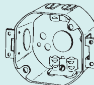
560LXE 1-1/2" Deep Plaster Ears
