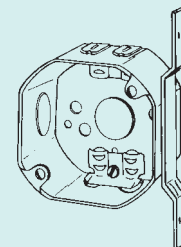
560LVB 1-1/2" Deep Plain Vertical bracket set back 5/8"
