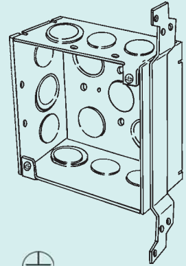
4SD-1 2-1/8" Deep, Welded
