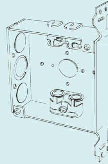
4SXVB-EK-PL 1-1/2" Deep, Welded Plain vertical bracket
