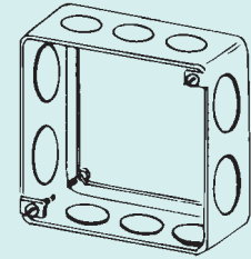
4SES Combo Extension-Thru-Ring 1-1/2" Deep, Drawn Top: Two 8-32 screws Bottom: Two 8-32 screws and two slide-on slots
