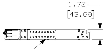
← 2X MOUNTING BRACKET (SEE NOTE 4)
