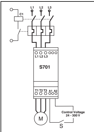
Figure 7. Input Controlled Soft Start *
