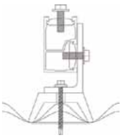
Corrugated Roof Straddle Block
