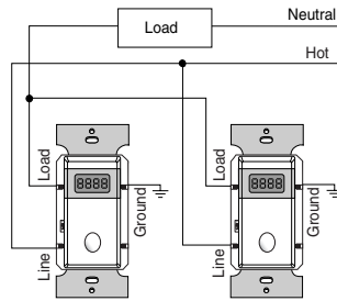
Three-way wiring
