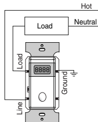
Single-switch wiring
